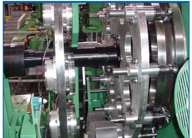
Turret upgraded with square clamp rods
