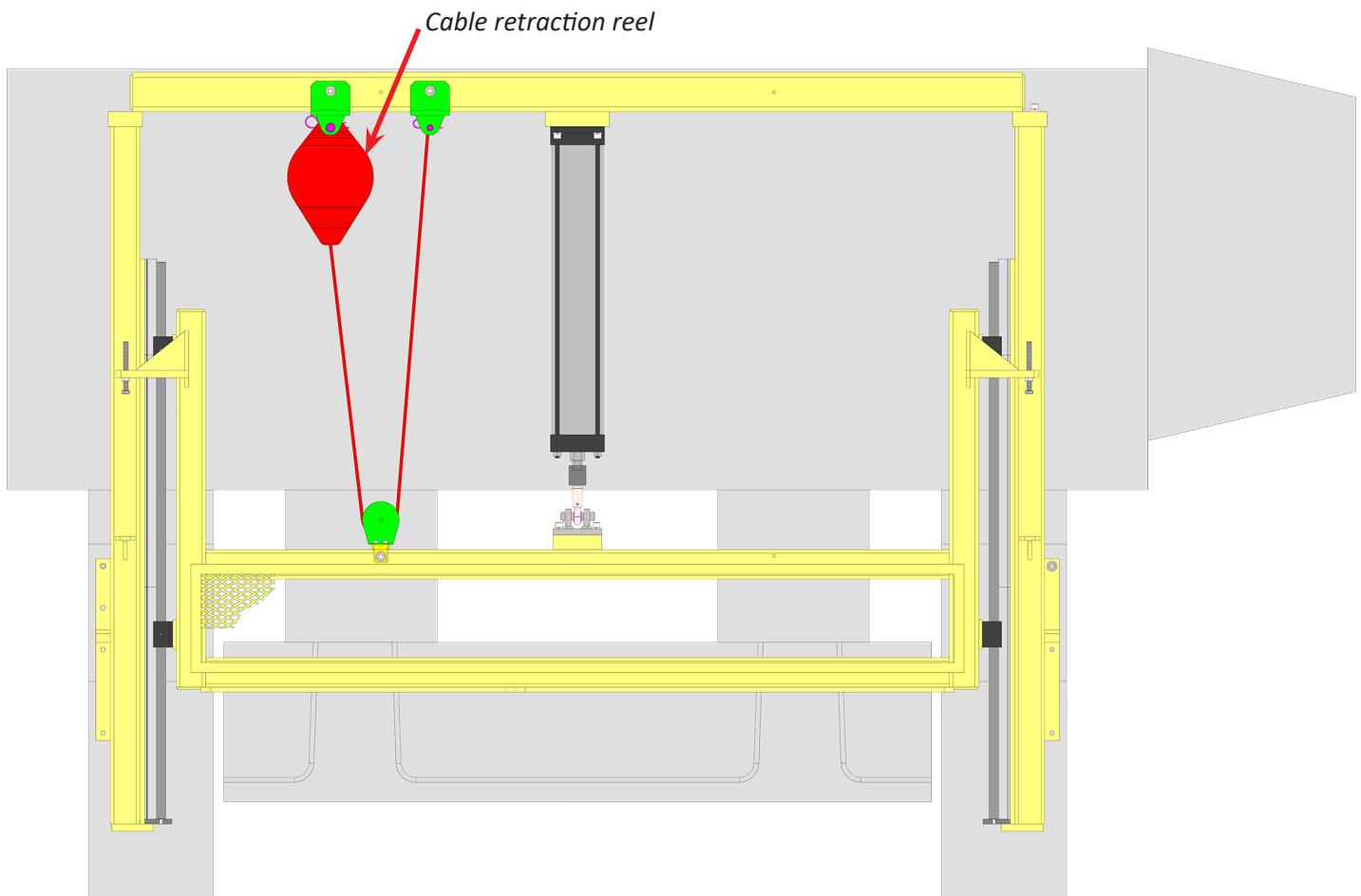
Previous belt design guard fall arrest assembly
