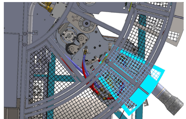
Individual sliding doors with safety interlocks on the front side allow easy access to the 8 inker units
