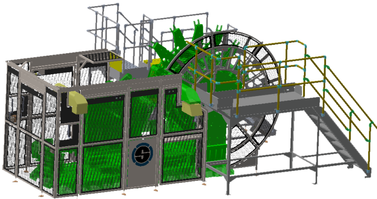
Operator side of Rutherford Decorator showing new perimeter guard package and the Stolle front platform
