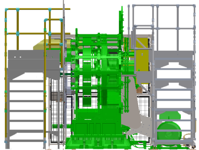
Print section end of machine showing print section front platform (left) and new rear platform (right)
