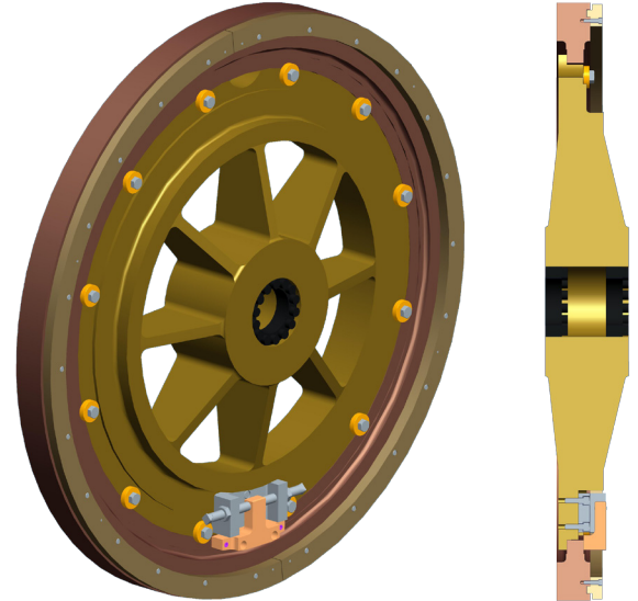
Redesigned bull gear for the 6-Color Rutherford Decorator
