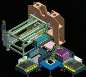
Robotic Sheet Feed Shell System
