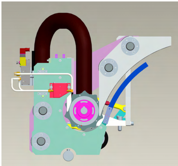
Vertical Vacuum Infeed model (left) and installed on Rutherford Decorator (right)
