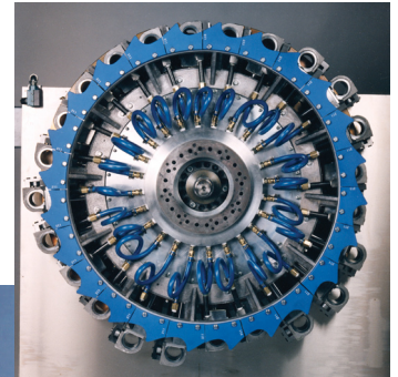
The Rutherford Linear Roller Spindle Disc
