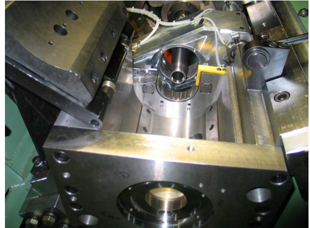
The redesigned Ragsdale tool pack cradle shown opened (above) and closed (below)
